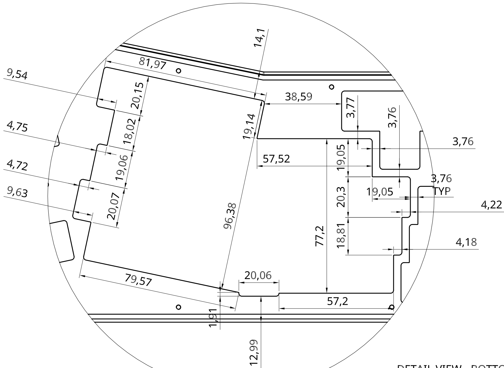
DETAIL VIEW - BOTTOM CUTOUT DIMENSION DETAILS
