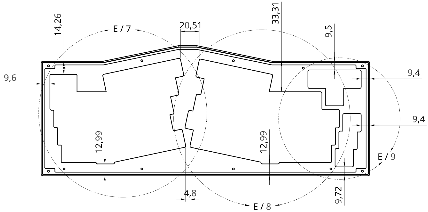
PLAN VIEW - BOTTOM CUTOUT DIMENSION DETAILS
