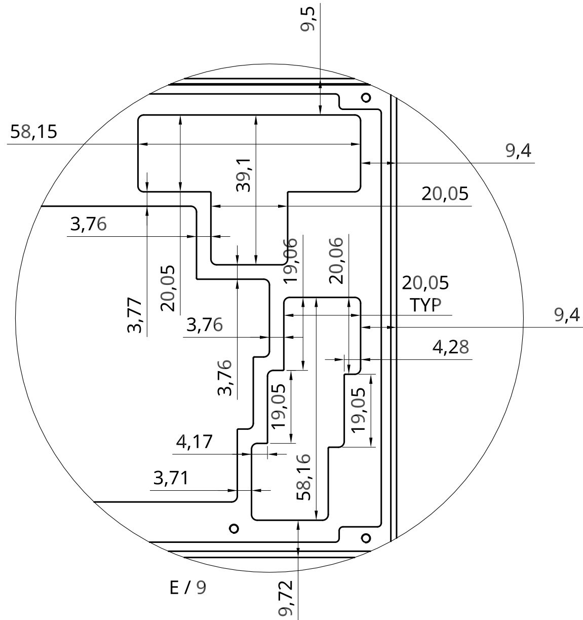
DETAIL VIEW - BOTTOM CUTOUT DIMENSION DETAILS
