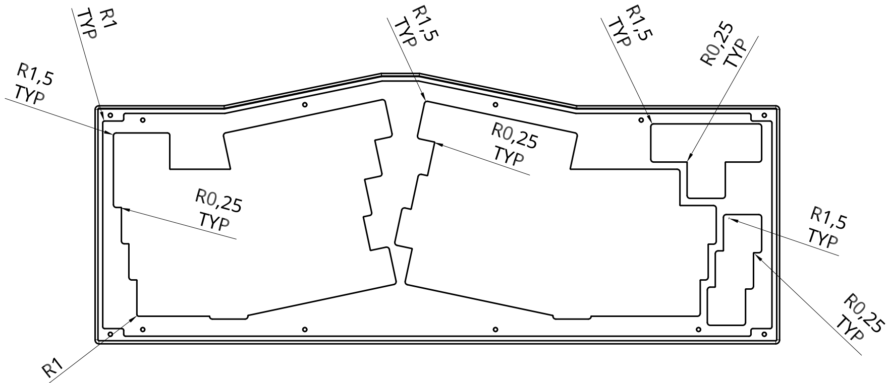
PLAN VIEW - BOTTOM RADII INNER FLANGE AND CUTOUTS
