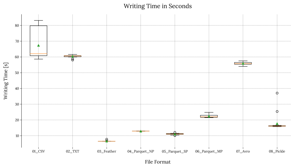
FIGURE 1.2: BOXPLOT DENOTING THE DISTRIBUTION OF 20 TRIALS OF WRITING TIMES FOR EACH FILE FORMAT
