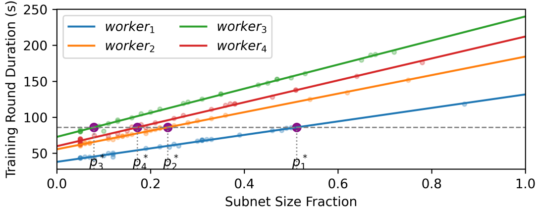
FIGURE 4.2: Duration of a single training round vs. the fraction of partitionable residual blocks assigned to each worker in ResNet-101. Each curve represents a different worker, illustrating how training round duration scales linearly with the number of residual blocks. P = \langle p_1^*, \dots, p_4^* \rangle is the optimal partitioning distribution vector used in the ideal initialization baseline throughout the training.
