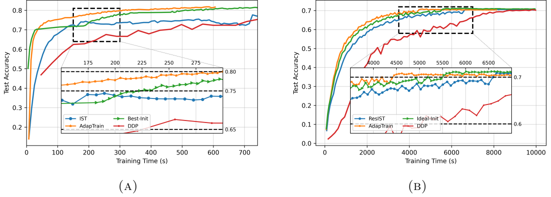
FIGURE 5.4: Comparison of test accuracy over training time for: (A) 3-Layer FCNN and (B) ResNet-101
