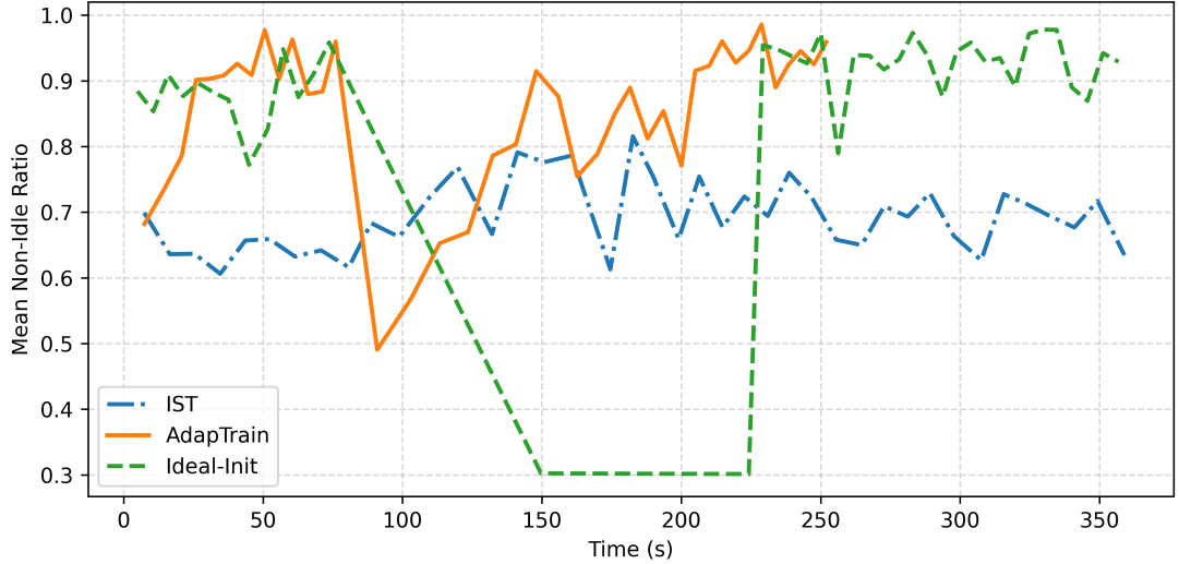
FIGURE 5.3: Mean non-idle ratio across workers throughout training a 3-layer FCNN on a public cloud environment.
