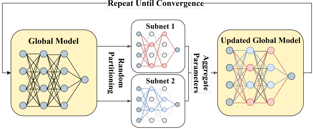
FIGURE 2.2: Overview of a training round in the Independent Subnet Training (IST) approach with two workers. Adopted from [14].
