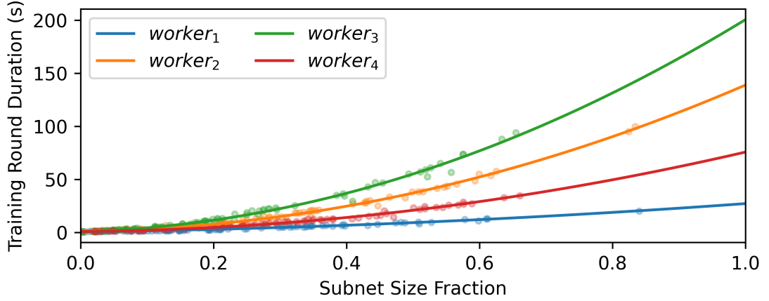
FIGURE 4.1: Duration of a single training round vs. the fraction of model neurons assigned to each worker in a fully connected neural network. Each curve represents a different worker, illustrating how training round duration increases quadratically with subnet size.
