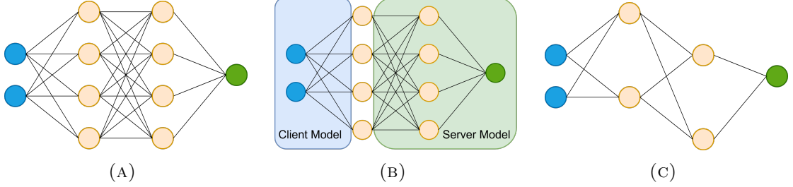
FIGURE 2.1: (A) In model-sharing algorithms, the entire model is sent to every participating client for local training. (B) In Split Learning, the model is divided horizontally across layers, with different segments handled by the client and the server. (C) In Partial Training, the model is partitioned vertically, meaning each client trains a smaller but complete version of the model that can be trained end-to-end. Adopted from [19].
