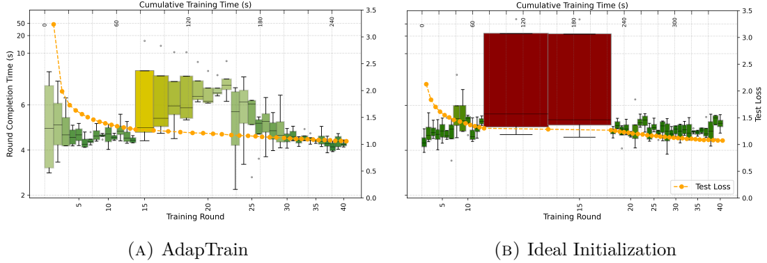
FIGURE 5.5: Distribution of training round completion times across workers during the first 40 training rounds for (A) AdapTrain and (B) Ideal-Initialization approach, both training a 3-layer fully connected neural network on Google Speech Commands. The top axis illustrates the cumulative training time, while the bottom axis shows the training round. The left y-axis uses a piecewise linear scale to display the main trend and occasional spikes, while the right y-axis represents the test loss. Each box plot’s width represents the round duration, emphasizing the variability across rounds, and the colour gradient (green to red) visually encodes the round duration, with green indicating shorter rounds and red representing longer ones.
