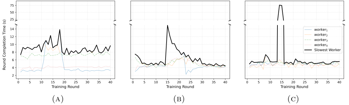
FIGURE 5.2: Training rounds durations across workers throughout training a 3-layer FCNN on public cloud environment using (A) IST (B) AdapTrain (C) Ideal-Initialization. The broken y-axis helps illustrate the main trend of round completion times throughout training and sudden, significant spikes. The black curve indicates the last worker to complete training at each training round.
