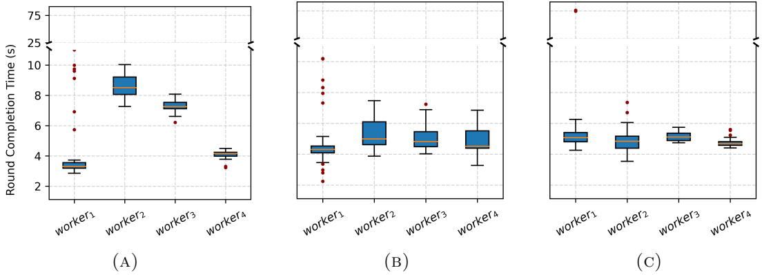
FIGURE 5.1: Distribution of training round completion times for each worker throughout training a 3-layer FCNN on public cloud environment using (A) IST (B) AdapTrain (C) Ideal-Initialization. The broken y-axis helps illustrate both the main trend of round completion times throughout training as well as outliers.
