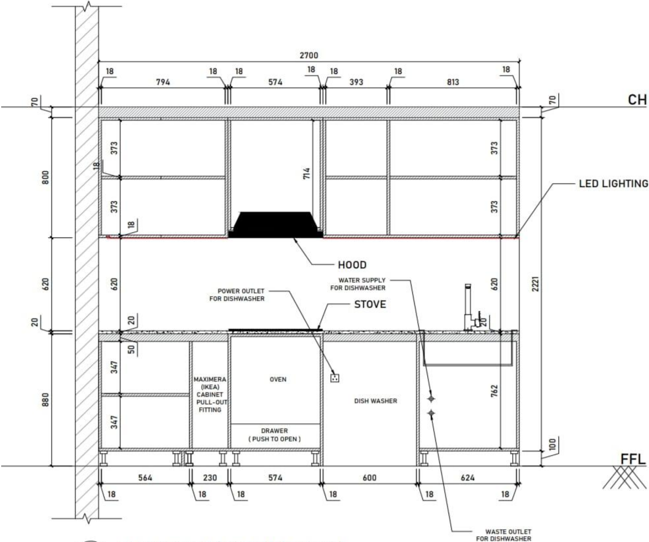
3.1 ELEVATION B ( INTERNAL VIEW ) SCALE 1:40
