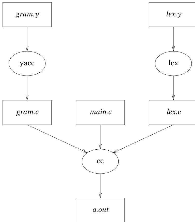
Figure 2: Compilation process.
