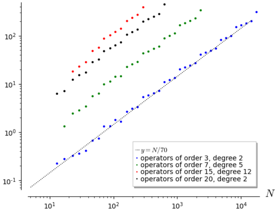
Figure 2.1: Computation time for random operators of varying orders and degrees
