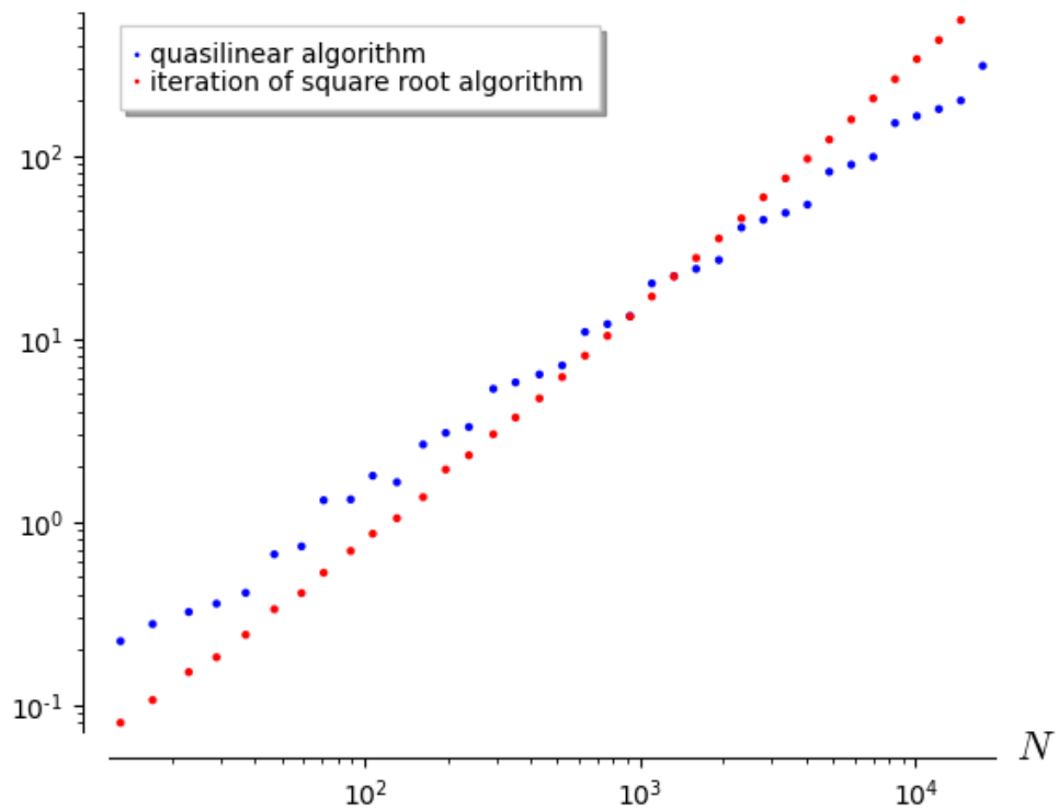
Figure 2.2: Comparison between iteration of [BCS14]’s algorithm and our algorithm times for operators of order 3 and degree 2
