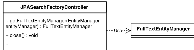
Figure 12: JPASearchFactoryController
