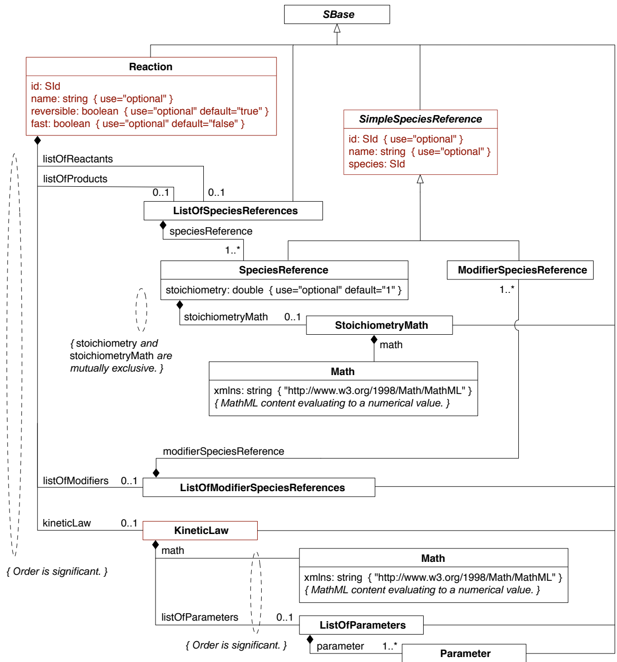
Figure 21: The definitions of classes Reaction , KineticLaw , SpeciesReference , ModifierSpeciesReference , as well as the container classes ListOfSpeciesReferences , ListOfModifierSpeciesReferences , and ListOfParameters . Note that SimpleSpeciesReference is an abstract class used only to provide some common attributes to its derived classes. The class Parameter is defined in Section 4.9.
