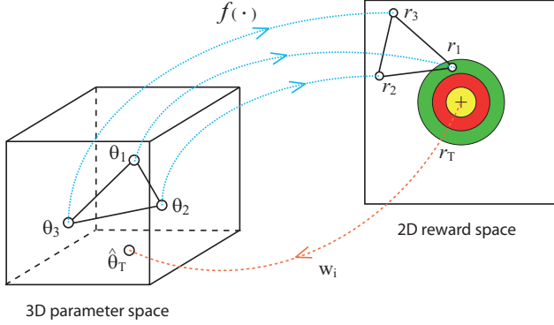
Fig. 3. The conceptual idea underlying the ARCHER algorithm.
