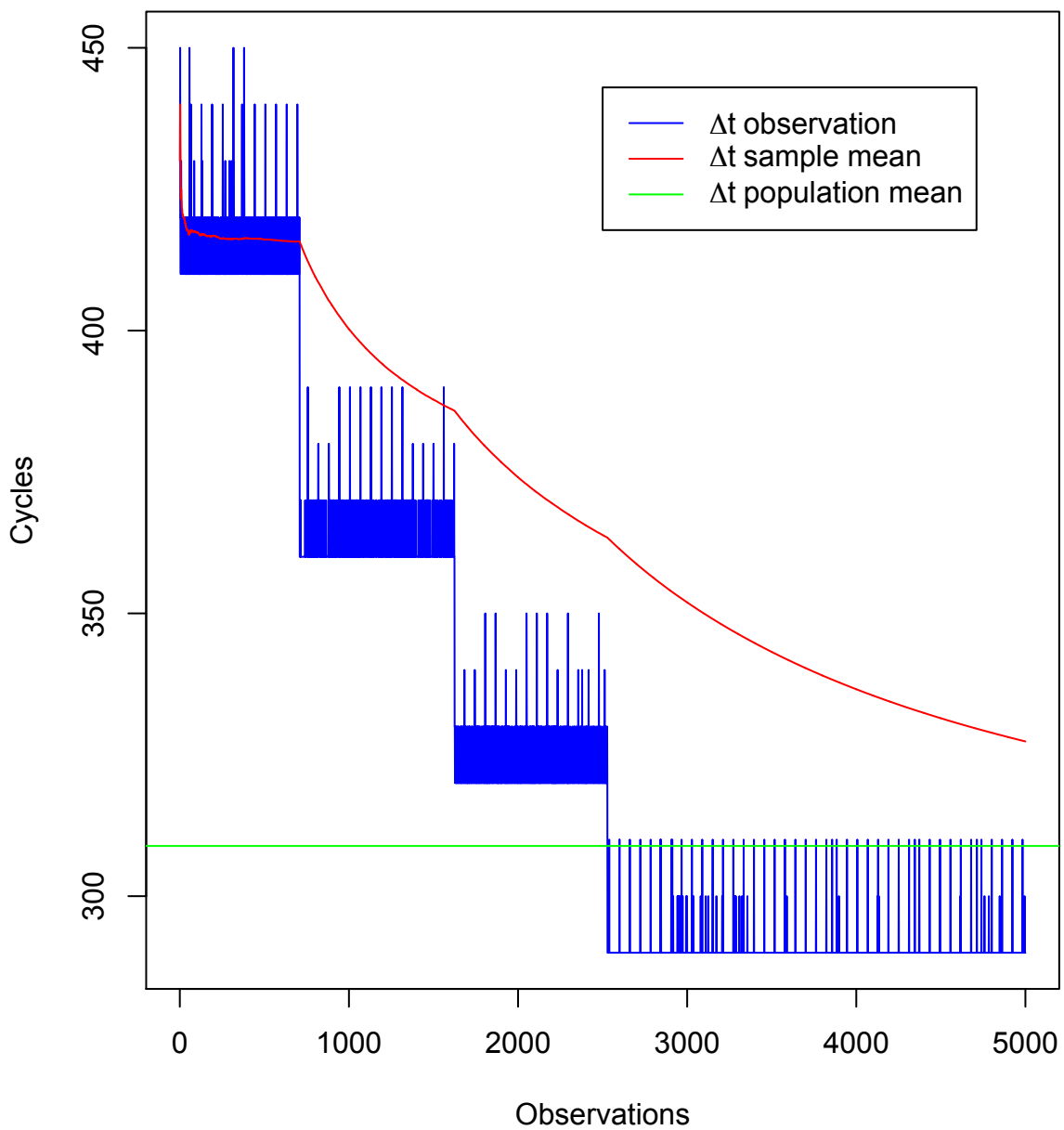
Time series of Intel rdtsc \Delta t
