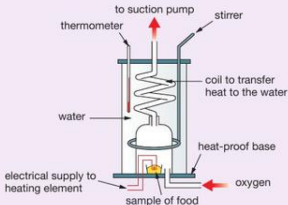
► Figure 4.12 A food calorimeter
