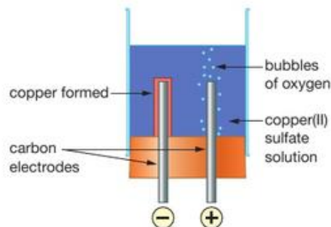
▲ Figure 10.8 Electrolysis of copper(II) sulfate solution using inert electrodes produces copper at the cathode and oxygen gas at the anode.
