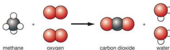
▲ Figure 5.5 A balanced equation for the reaction between methane and oxygen.
