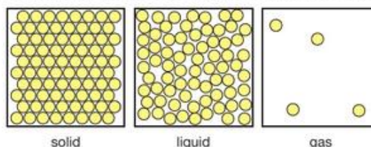
▲ Figure 1.4 The arrangement of particles in different states of matter
