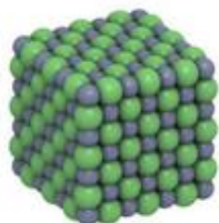
▲ Figure 7.17 A model of a small part of a sodium chloride crystal
