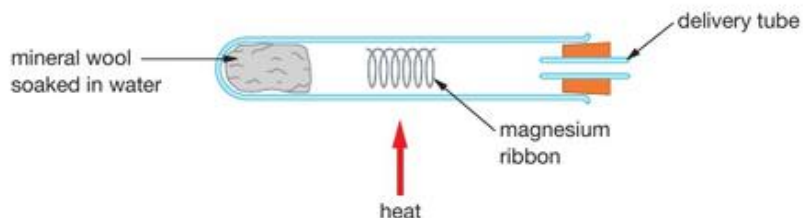
▲ Figure 14.10 Magnesium reacting with steam
