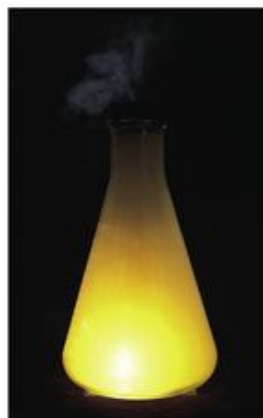
▲ Figure 12.4 Sodium burning in chlorine to produce sodium chloride.
