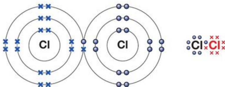
▲ Figure 8.7 Two ways of showing the covalent bonding in Cl_2
