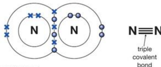
▲ Figure 8.16 N_2 has a triple bond
