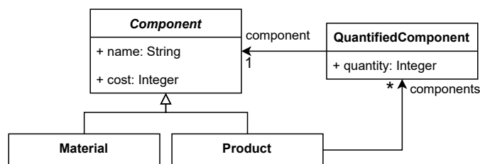
Fig. 1. Parts list class diagram
