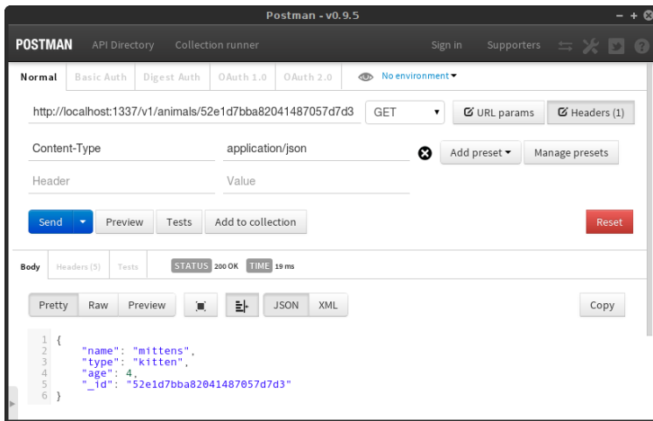
Figure 1.1: Postman Screenshot
