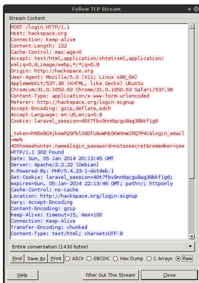
Figure 1.2: Wireshark Screenshot
