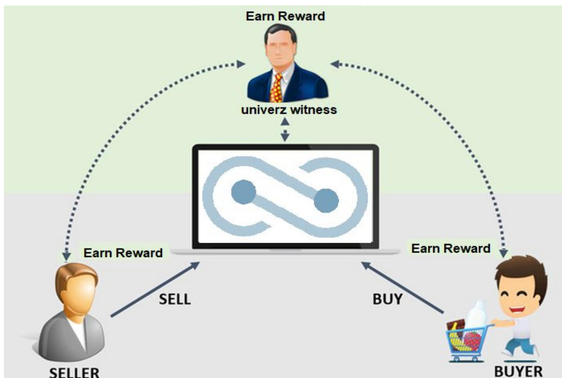
Figure 3: Reward System
