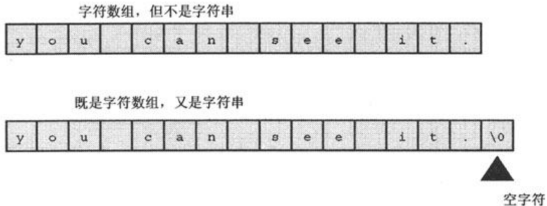
图6.6 字符数组和字符串
