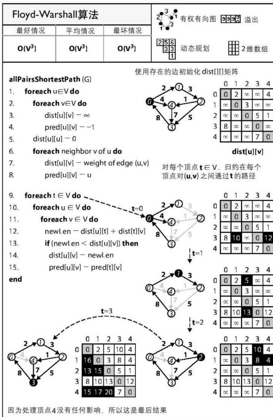
图 6-18 Floyd-Warshall详解
