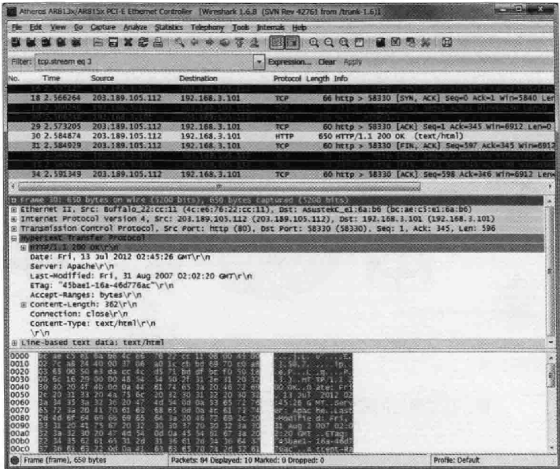
图: Wireshark ( http://www.wireshark.org/ )
