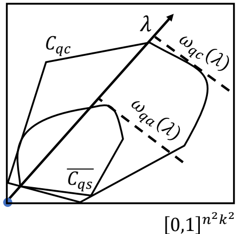
Figure 1: Separating convex sets
