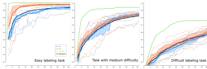
Fig. 4: The accuracy of labeling strategies depends on the complexity of the labeling task. The performance of all VIL results (orange) can at least compete with the performance of AL (blue), and RB (black). ULoP (green) substantially outperforms all remaining strategies. Dashed lines represent minimum and maximum performances, area dyed with decreased alpha is used to depict 25% and 75% quartiles.
