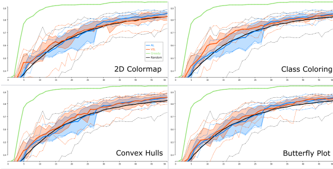
Fig. 6: Performance comparison of four VIL-support techniques (orange) with AL strategies (blue), RB (black), and ULoP (green) for a labeling task with medium difficulty ( PART 1 ). All VIL-support techniques have accuracies at least as high as AL and RB in earlier phases of the process. Convex hulls can compete with the AL performance for the entire observed process. ULoP (green) substantially outperforms all remaining techniques.
