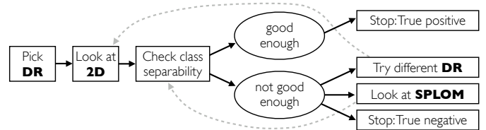
Fig. 8. A workflow model for guiding VE and DR technique choices in the DR exploration process.
