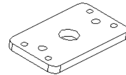
Gối đỡ UCFL - 204 Bracket for bearing holder
