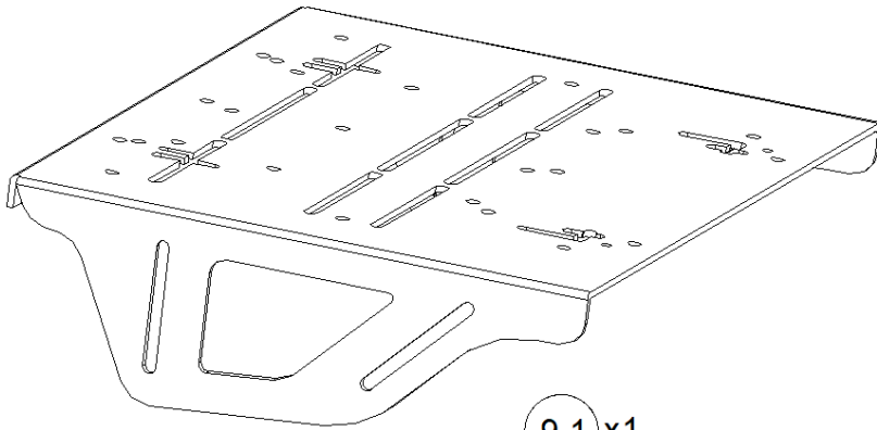
9.1 x1 Gá Pedal Pedal mount
