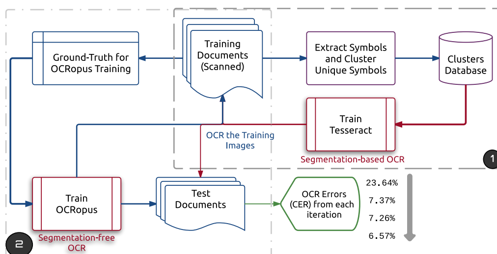
Figure 6.5: The process diagram of OCRoRACT system. In the first phase of process (shown in dashed box marked with '1'), unique symbols are extracted from the training corpus of scanned pages. These symbols are then used to train the Tesseract OCR system. The trained models obtained from the Tesseract are then used to generate semi-corrected GT information for the training of OCRopus OCR system. In the second phase (shown in dashed-dotted box marked with '2'), the OCRopus is iteratively used to train LSTM -based OCR models. The best model is subsequently applied first to the test data and then to improve the GT data, which is used in the next iteration.
