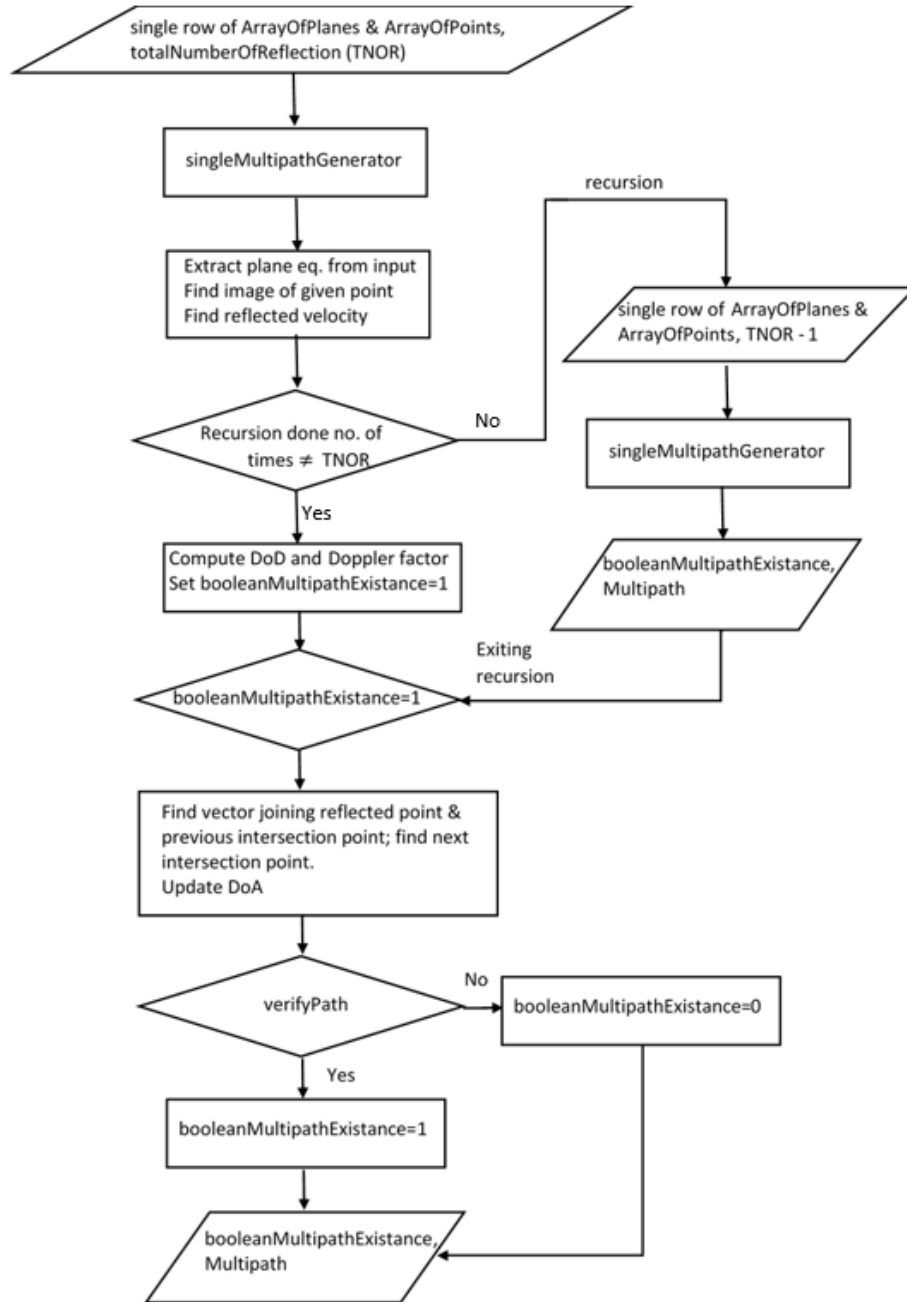
Figure 52: Flow chart of singleMultipathGenerator.m .
