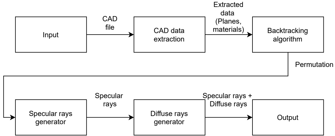
Figure 10: Step-by-step procedure of the NIST Q-D Channel Realization Software.
