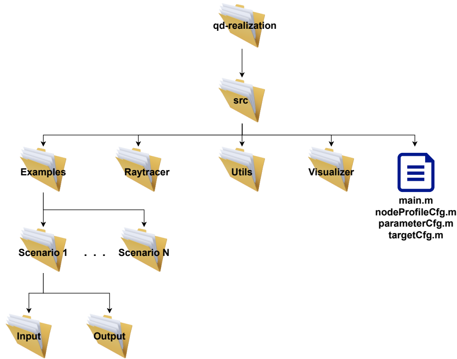
Figure 11: Directory structure of the NIST Q-D Channel Realization Software.
