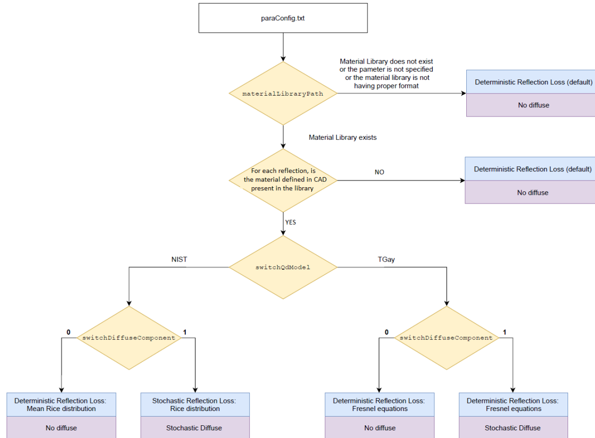
Figure 36: Flowchart of the different Q-D models implemented in the NIST Q-D Channel Realization Software.
