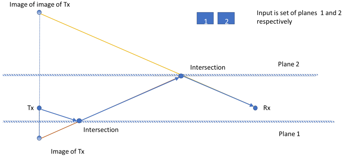
Figure 50: Method of images for a scenario with an input of two planes.
