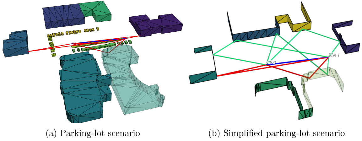
Figure 26: Parking-lot scenarios
