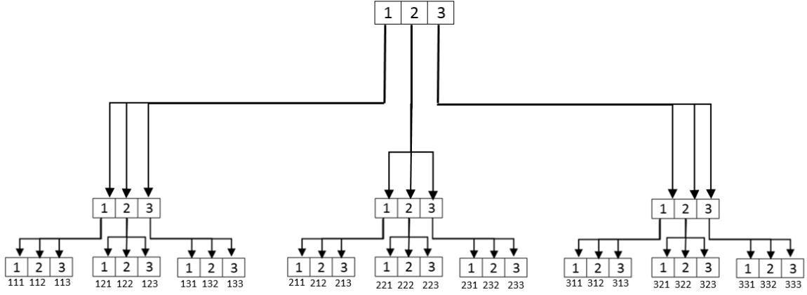
Figure 42: A recursive tree consists of three generations for a set 1,2,3. The last line shows all the combinations after traversing through every path in the tree.
