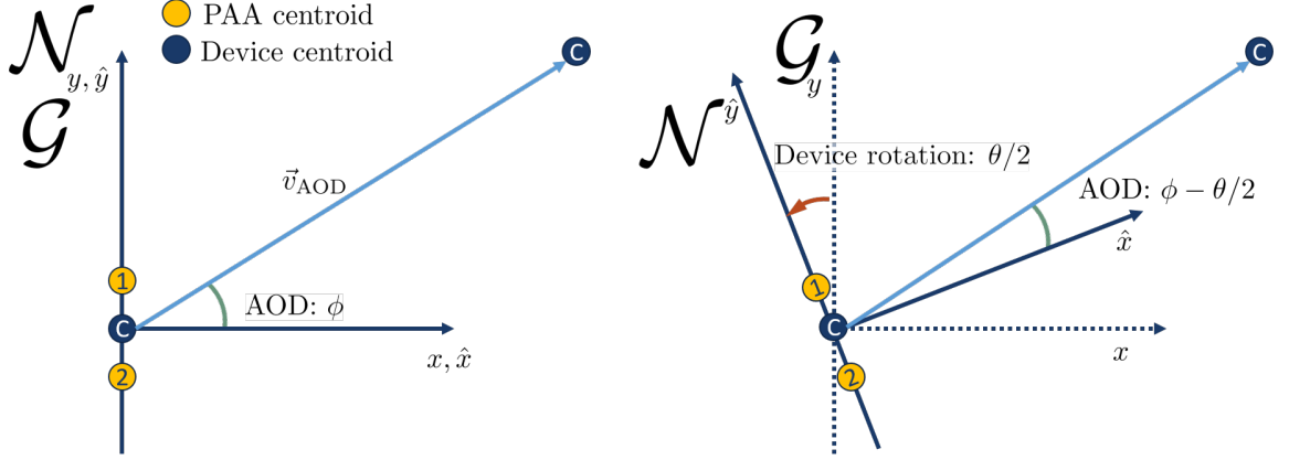
Figure 8: The point rotation is used to model the device rotation, which brings the PAAs in a different position in the global frame. The frame rotation is used to transform AoA and AoD from global to local coordinates.
