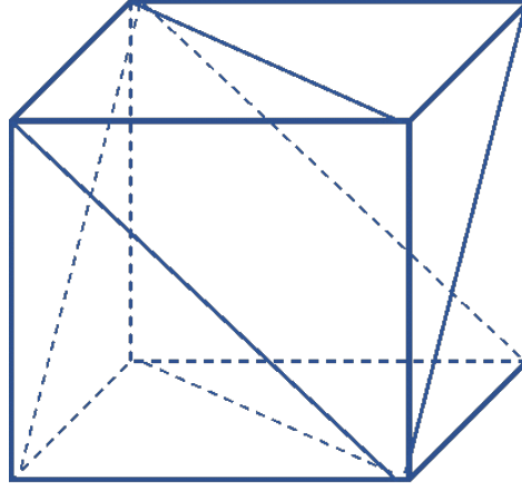
Figure 37: A cube is described by 12 triangles in the AMF file format.
