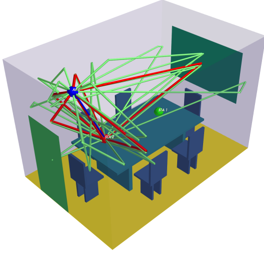
(a) Conference Room Scenario.
