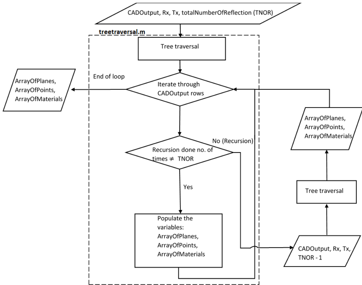
Figure 45: Flow chart of backtracking algorithm.
