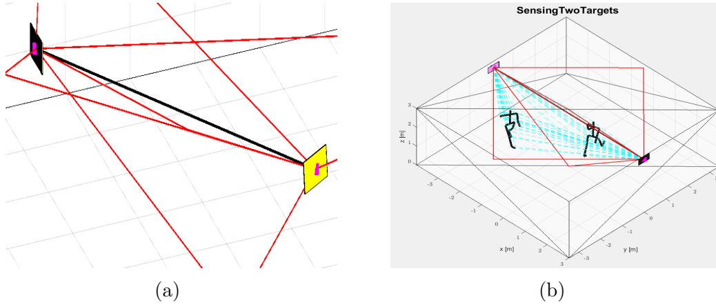
Figure 19: (a) PAA orientation at each node, which can be changed over time due to node rotation. (b) Target visualization in the scenario.
