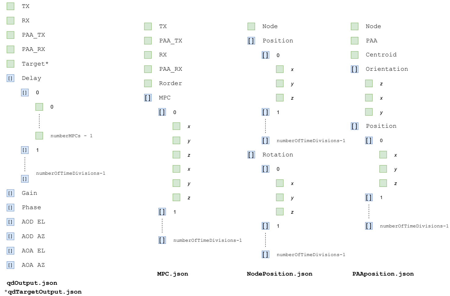
Figure 17: Visualizer JSON files.
