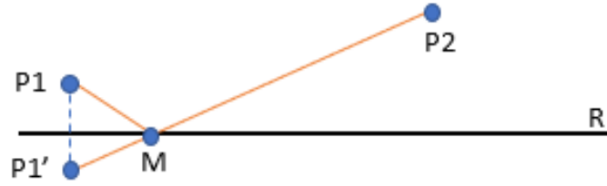
Figure 49: Reflected path between points P1 , P2 and reflecting plane R .
