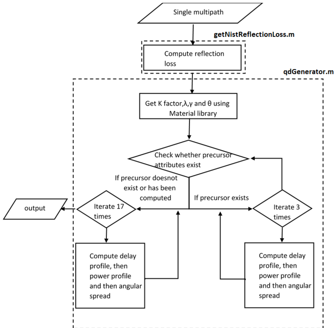
Figure 35: Flow chart of NIST Q-D model.
