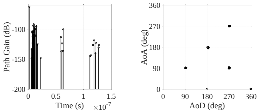
Figure 4: Space-time point-to-point DDIR.
