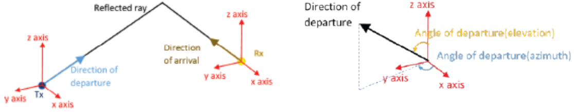
Figure 5: (Left) Reflected ray and its direction of arrival and departure vectors. (Right) The direction of departure is decomposed into azimuth and elevation planes.
