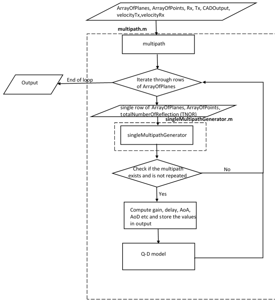
Figure 51: Flow chart of multipath.m .
