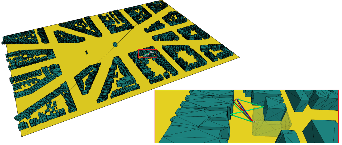
Figure 31: City block scenario where one node is attached to a building and other node is mobile on the ground.
