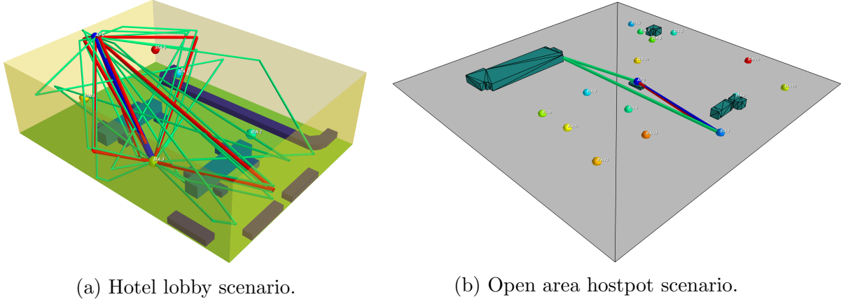
Figure 29: Hotel Lobby and Open Area hotspot scenarios
