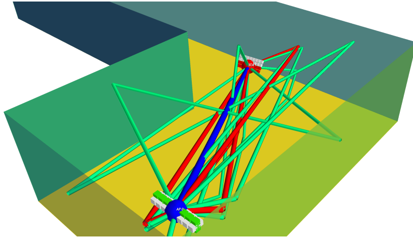
Figure 24: L-Room scenario with multiple PAAs and rotation
