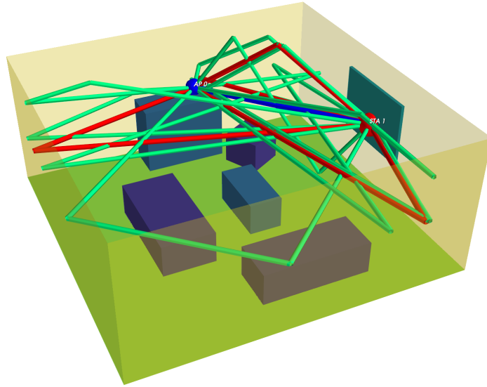
Figure 27: Living-room scenario.
