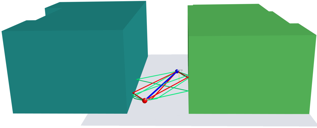
Figure 28: Street-canyon scenario.
