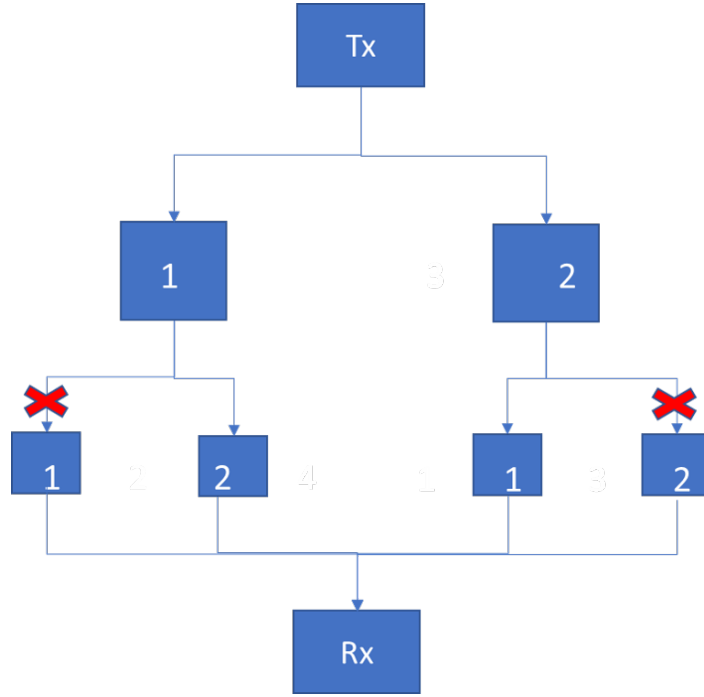
Figure 44: Schematic diagram of a Tree describing the backtracking algorithm.
