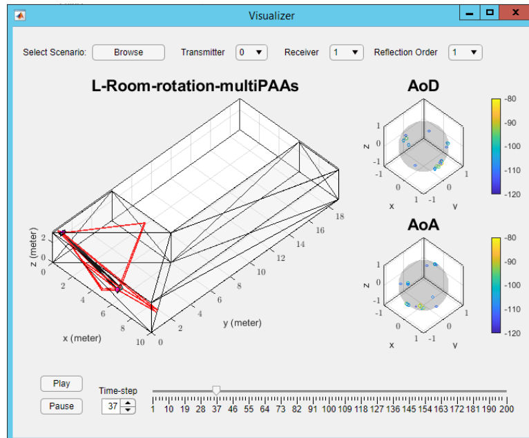
(b) Scenario with multiple PAAs per device
