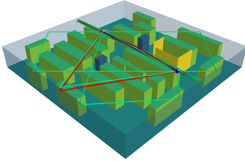
Figure 25: Data center scenario where both nodes are placed on rack-tops.
