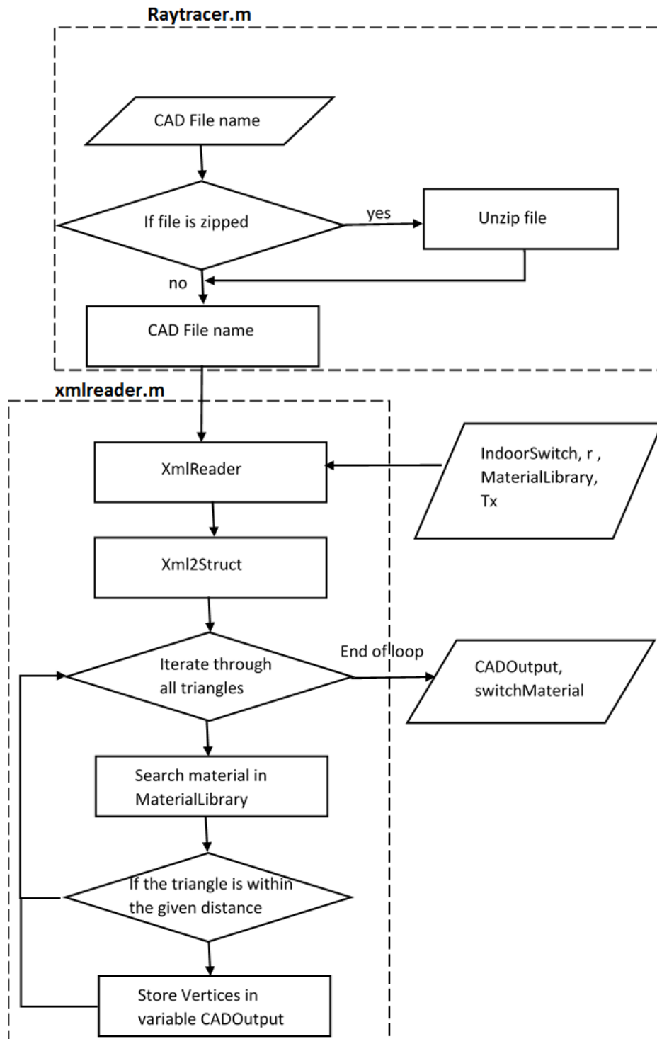
Figure 39: Flow chart of CAD extraction.
