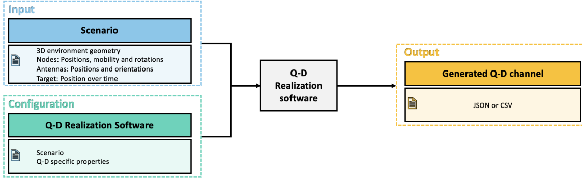
Figure 1: The NIST Q-D Channel Realization Software workflow.
