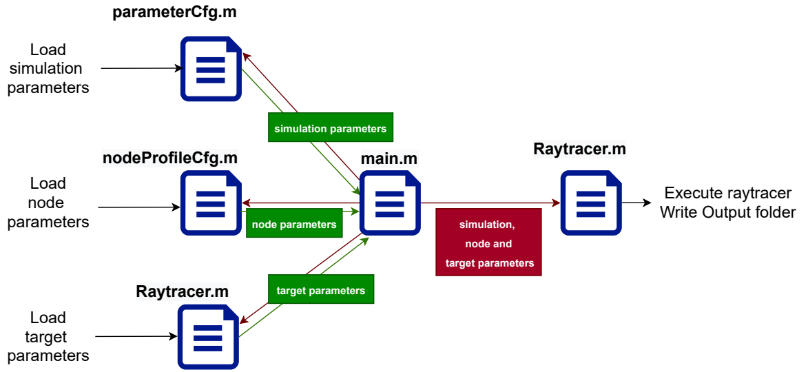
Figure 12: Main components of the NIST Q-D Channel Realization Software.
