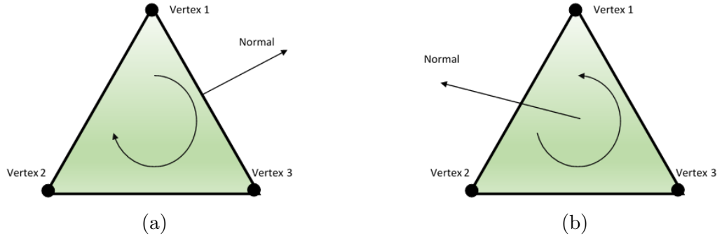
Figure 38: A triangle and its normal (a) when IndoorSwitch has a value of 1. The normal is taken in clockwise direction (b) when IndoorSwitch has a value of 0. The normal is taken in counterclockwise direction.
