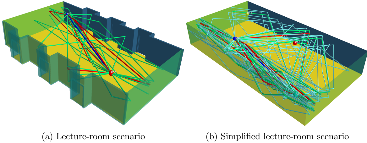
Figure 21: Lecture-room scenarios.
