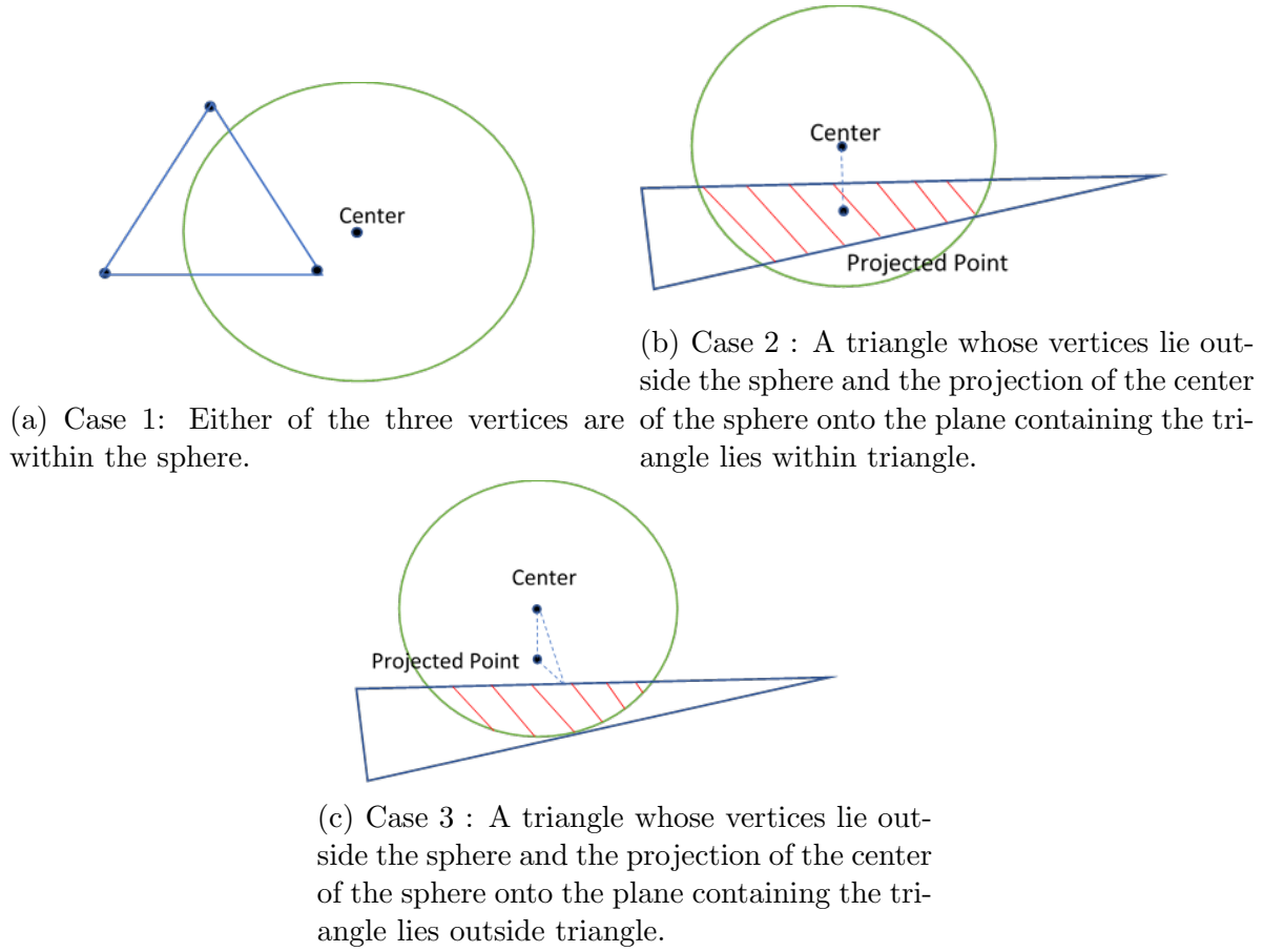
Figure 41: Three possible cases in which a triangle intersects the sphere.
