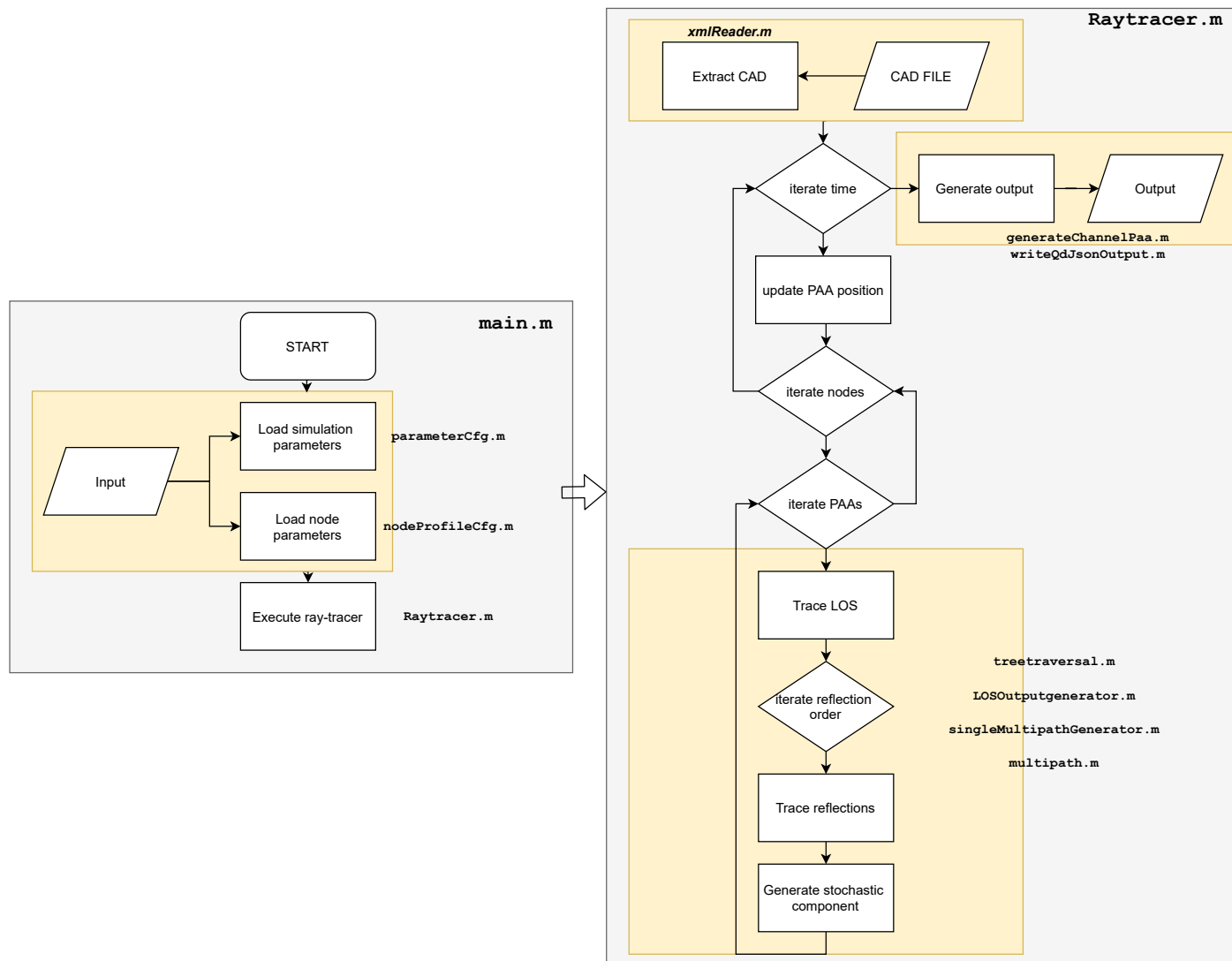
Figure 33: Flowchart of Raytracer.m.
