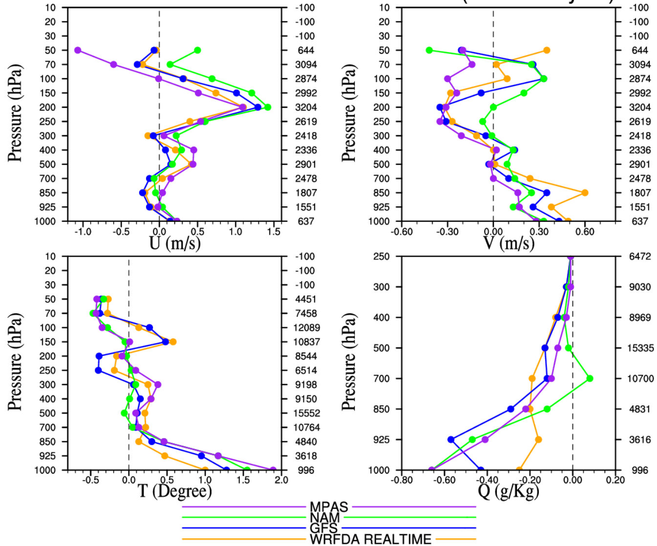
Bias Profiles 2017031800 - 2017040500 (24 hour Cycle)
