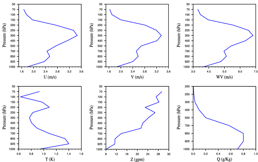
Absolute Bias 2017030200 - 2017030900 (24 hour Cycle)
