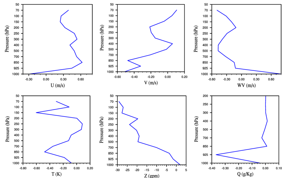
Bias 2017030200 - 2017030900 (24 hour Cycle)
