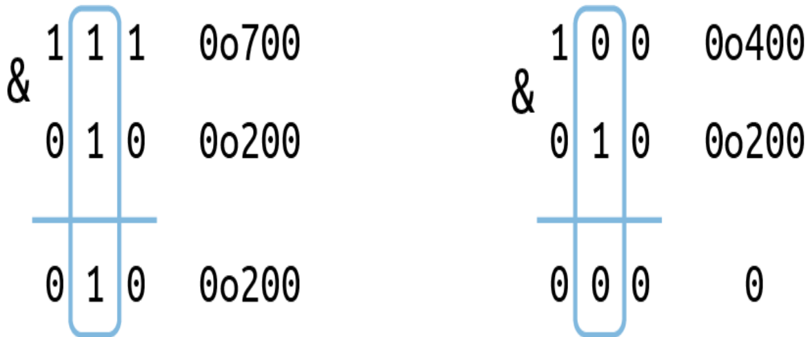
Figure 14-4. The binary AND operator & will set bit values in the result where both bits are set in the operands.
