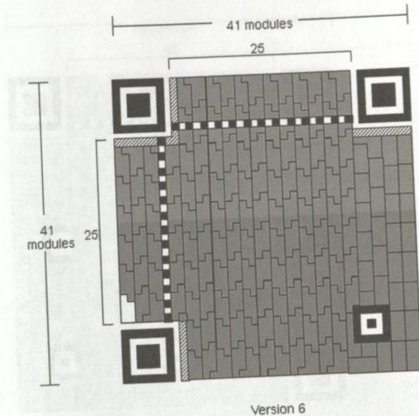
Figure 6 — Version 6 symbol
