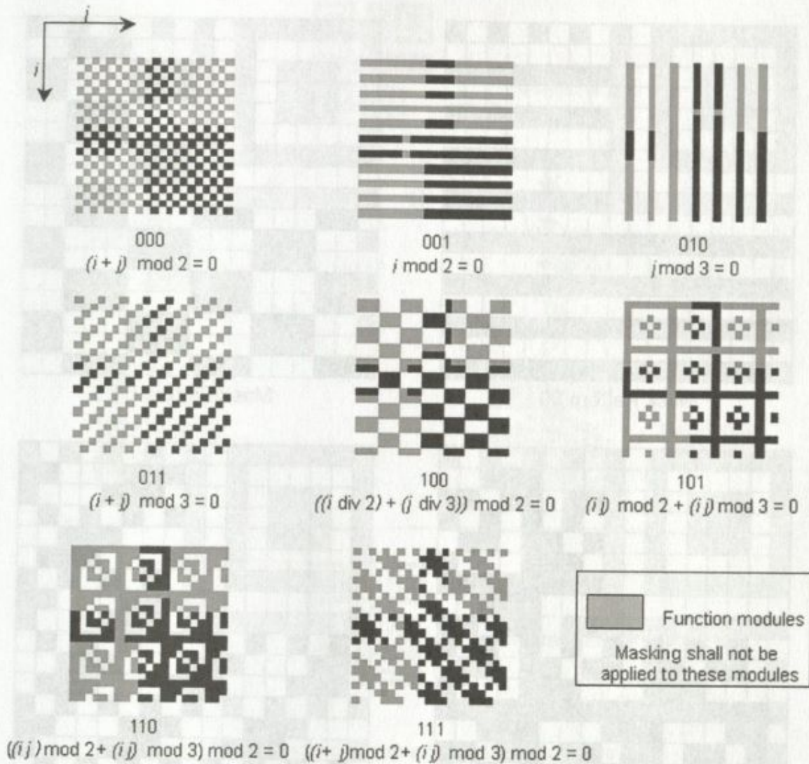
Figure 21 — Data mask patterns for version 1 symbol
