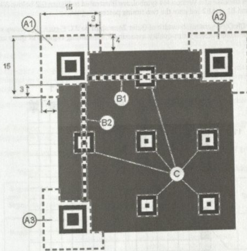
Figure G.1 — QR Code fixed pattern segments
