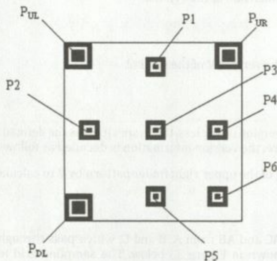
Figure 34 — Finder patterns and alignment patterns
