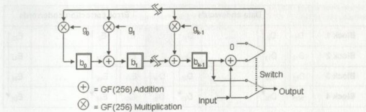
Figure 14 — Error correction codeword encoding circuit
