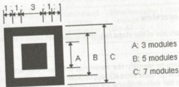
Figure 12 — Structure of finder pattern
