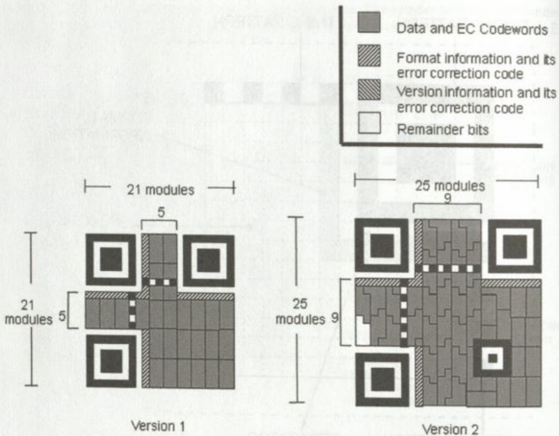
Figure 5 — Version 1 and 2 symbols
