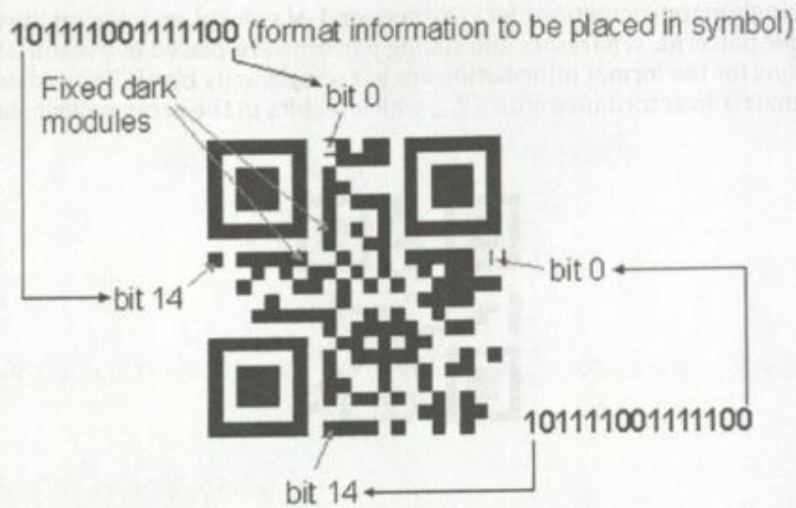
Figure I.2 — Final version 1-M symbol encoding 01234567
