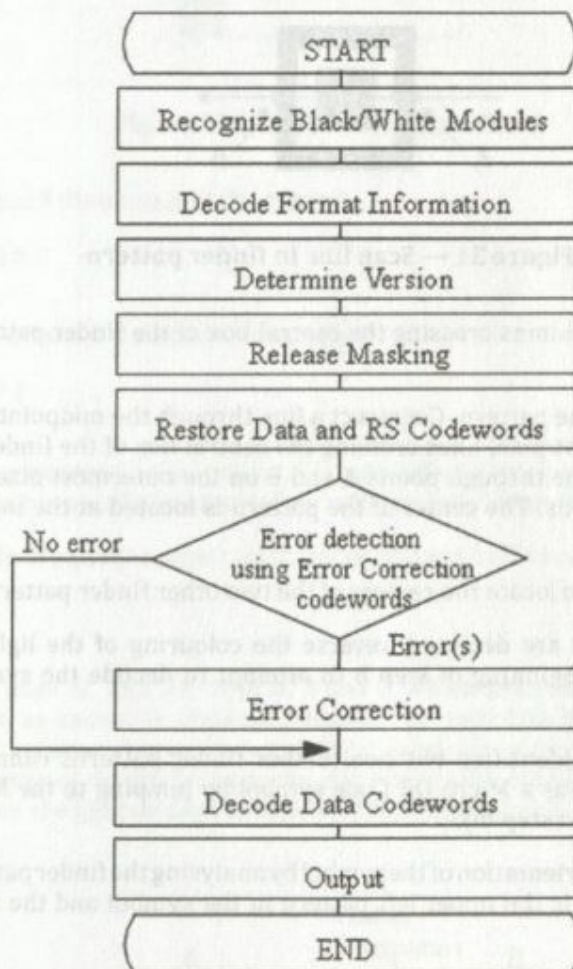
Figure 30 — QR Code decoding steps
