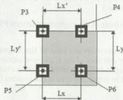
Figure 37 — Lower right area of symbol
