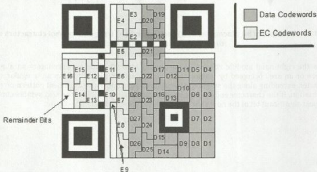
Figure 19 — Symbol character arrangement in version 2-M symbol
