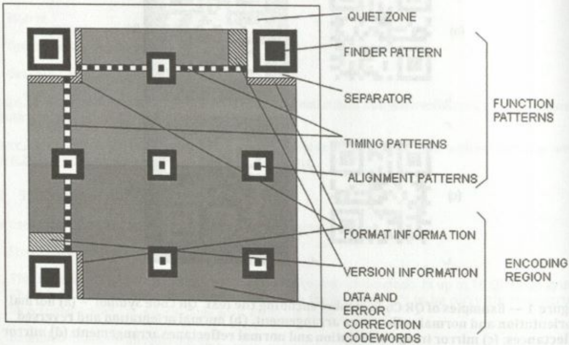
Figure 3 — Structure of a QR Code symbol
