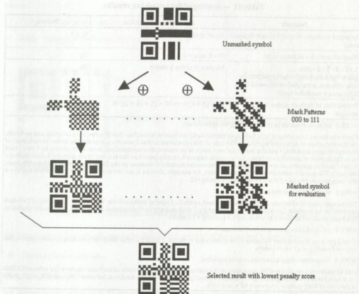
Figure 23 — Data masking simulation in QR Code symbols
