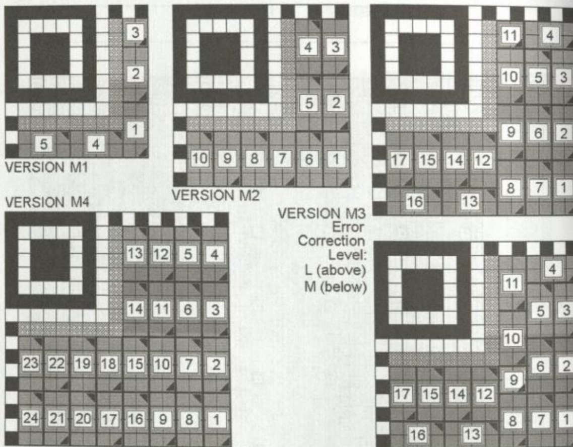
Figure 11 — Versions of Micro QR Code symbol
