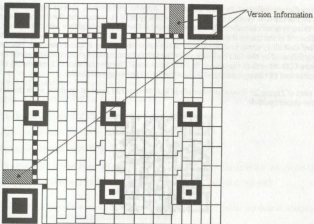
Figure 27 — Version information positioning
