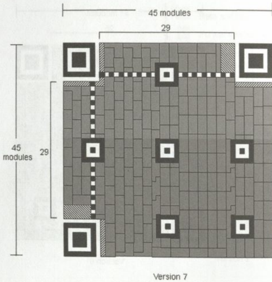
Version 7 Figure 7 — Version 7 symbol
