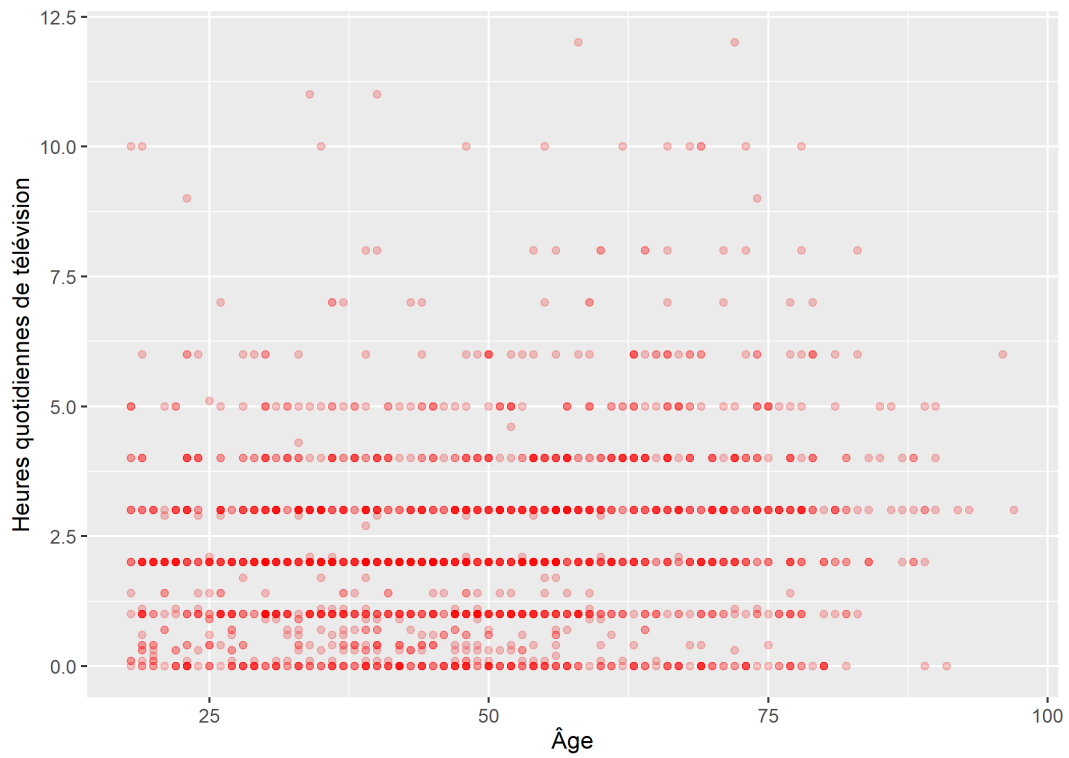
Figure 16. Nuage de points semi-transparents
