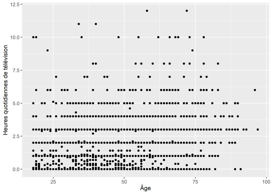
Figure 15. Nuage de points
