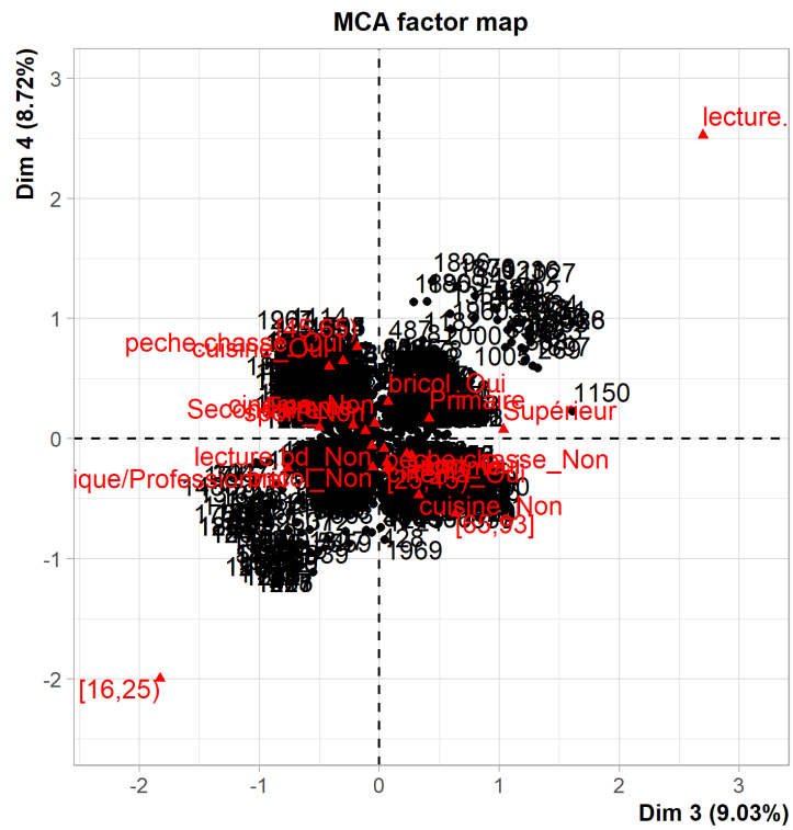
Figure 23. Plan factoriel (axes 3 et 4)
