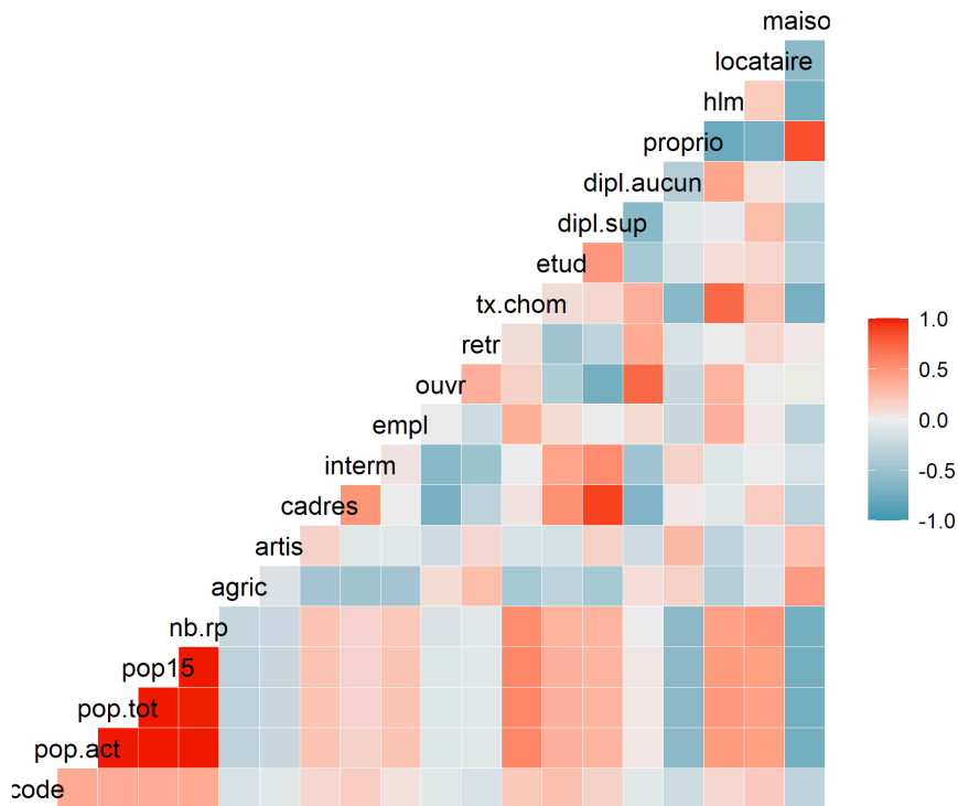
Figure 23. Matrice de corrélation
