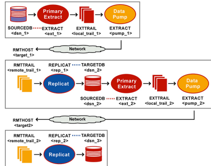
Figure 5-4 Cascading Configuration
